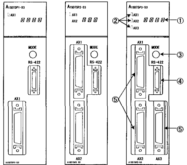
A1SD75P1-S3 front view A1SD75P2-S3 front view A1SD75P3-S3 front view
