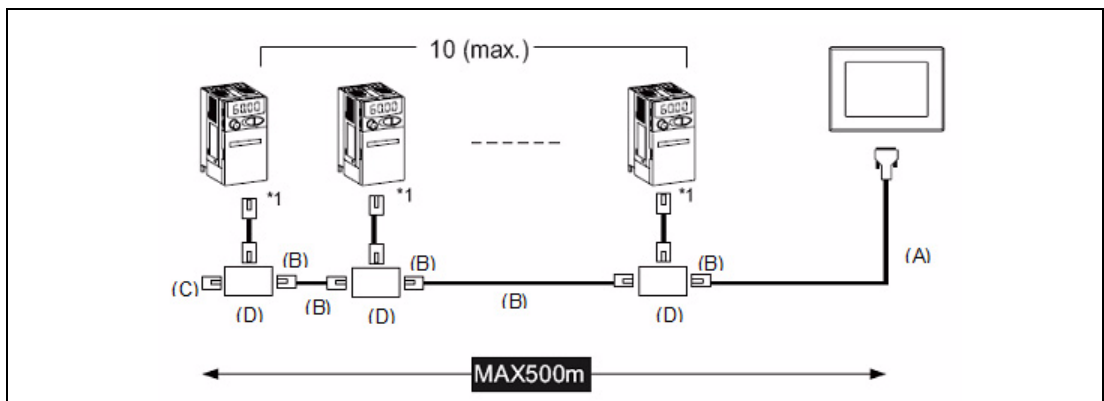
Fig. 2: Multi-drop connection
